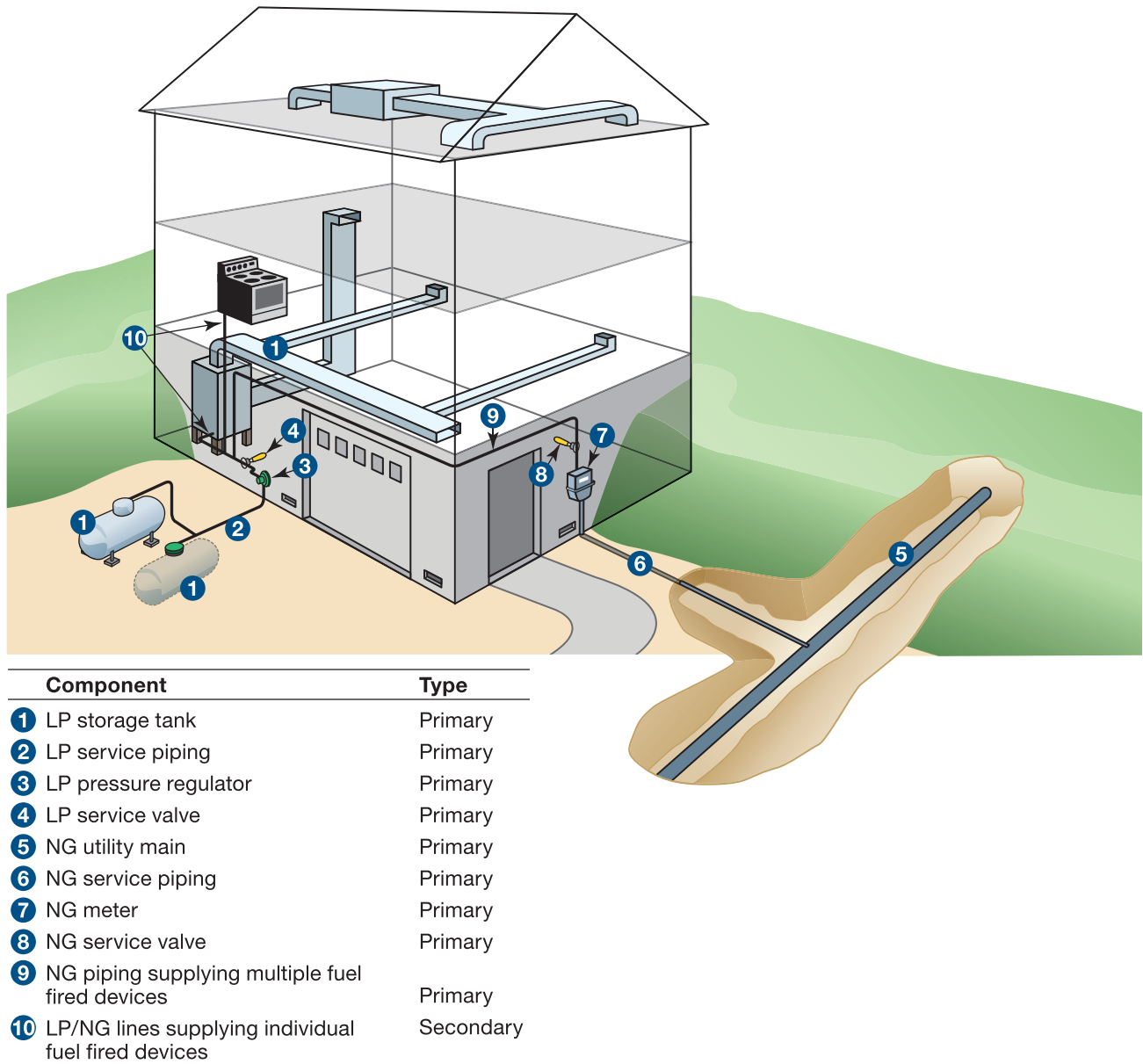
Figure 4-29. Typical elements of a residential flammable gas system – liquid propane (LP) with tank and pressure regulator (left side); natural gas (NG) with meter (right side).
