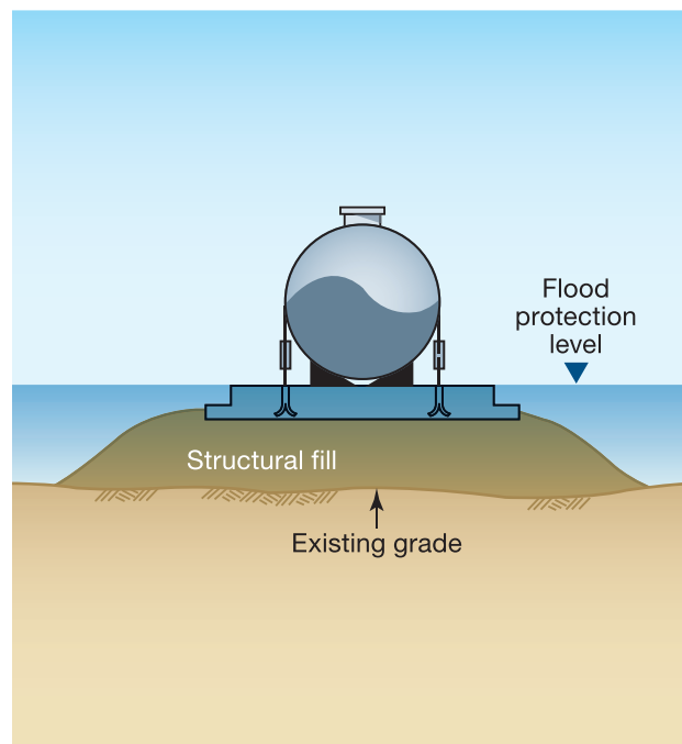
Figure 4-33. Fuel tank elevated on structural fill.
